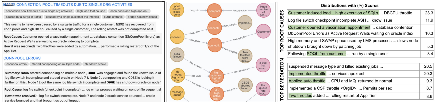
Figure 8: ICA output for Incident with Symptom “Connpool issues” (i) Incident Search Results (ii) Query Specific Causal Knowledge Subgraph (iii) Distribution of top detected root causes and resolutions (Highlighted spans show match with true)
